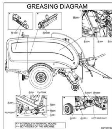
Greasing diagram ( CST00739 )
